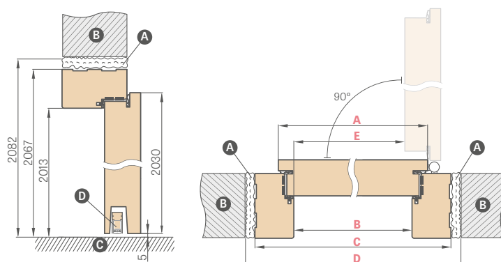
FIRE RATED DOOR FRAME CROSS-SECTION IN BASIC MASONRY
