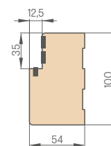
FIRE RATED FIXED DOOR FRAME CROSS-SECTION
