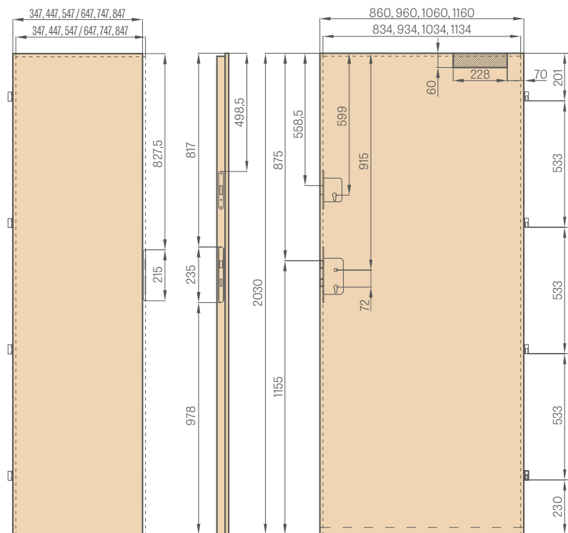
Side panel / inactive door leaf
