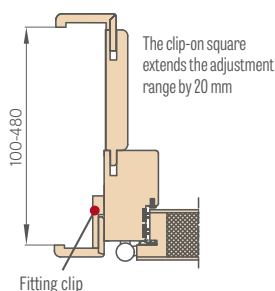
FIRE RATED DOOR FRAME CROSS-SECTION IN MASONRY AND WITH CLIP-ON SQUARE
